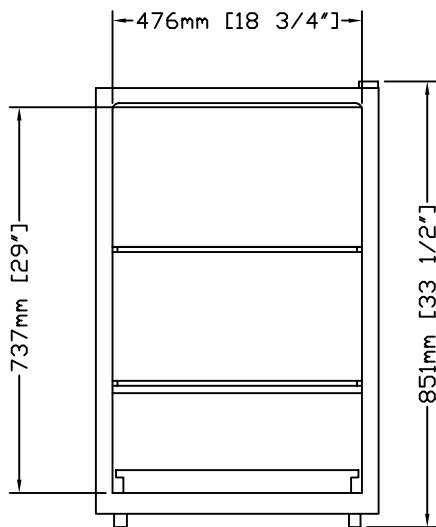
FRONT VIEW-SECTION
