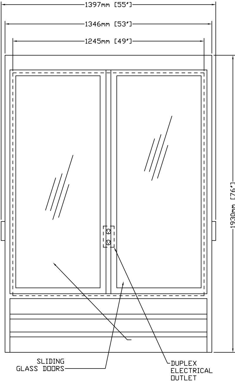
FRONT VIEW
