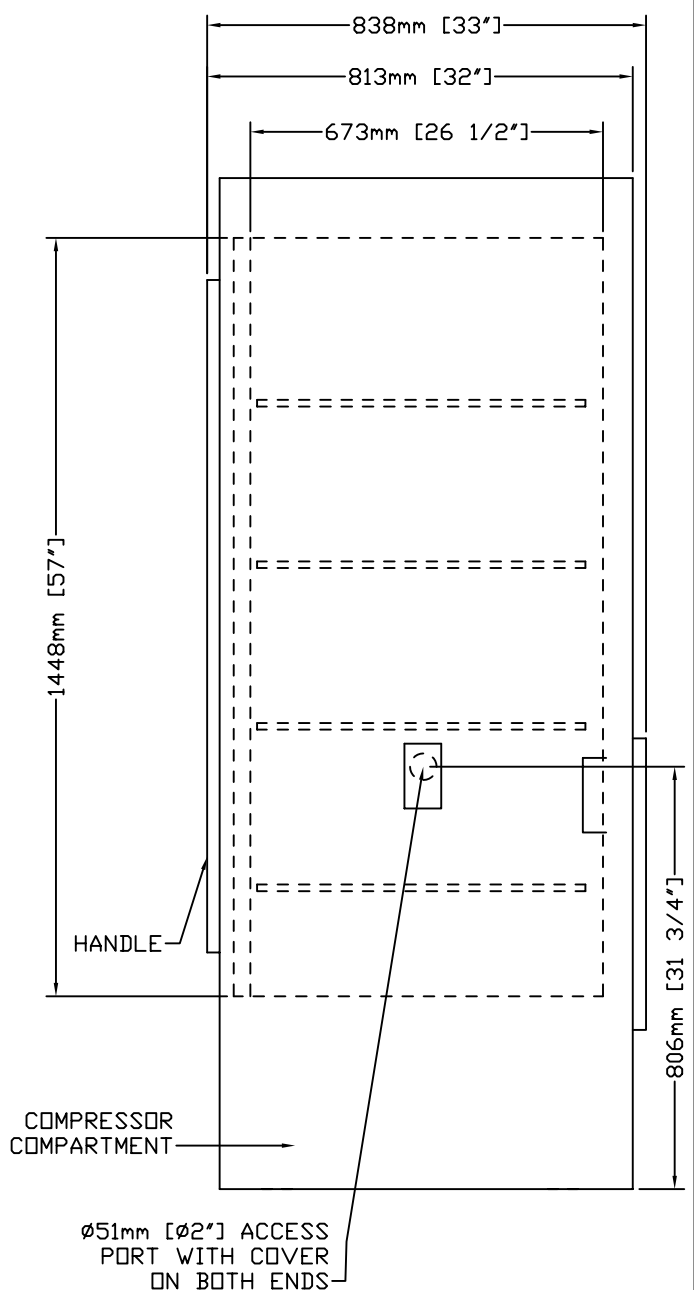
SIDE VIEW
