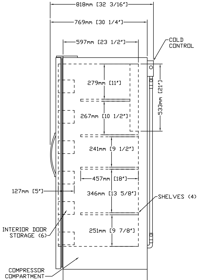
SIDE VIEW
