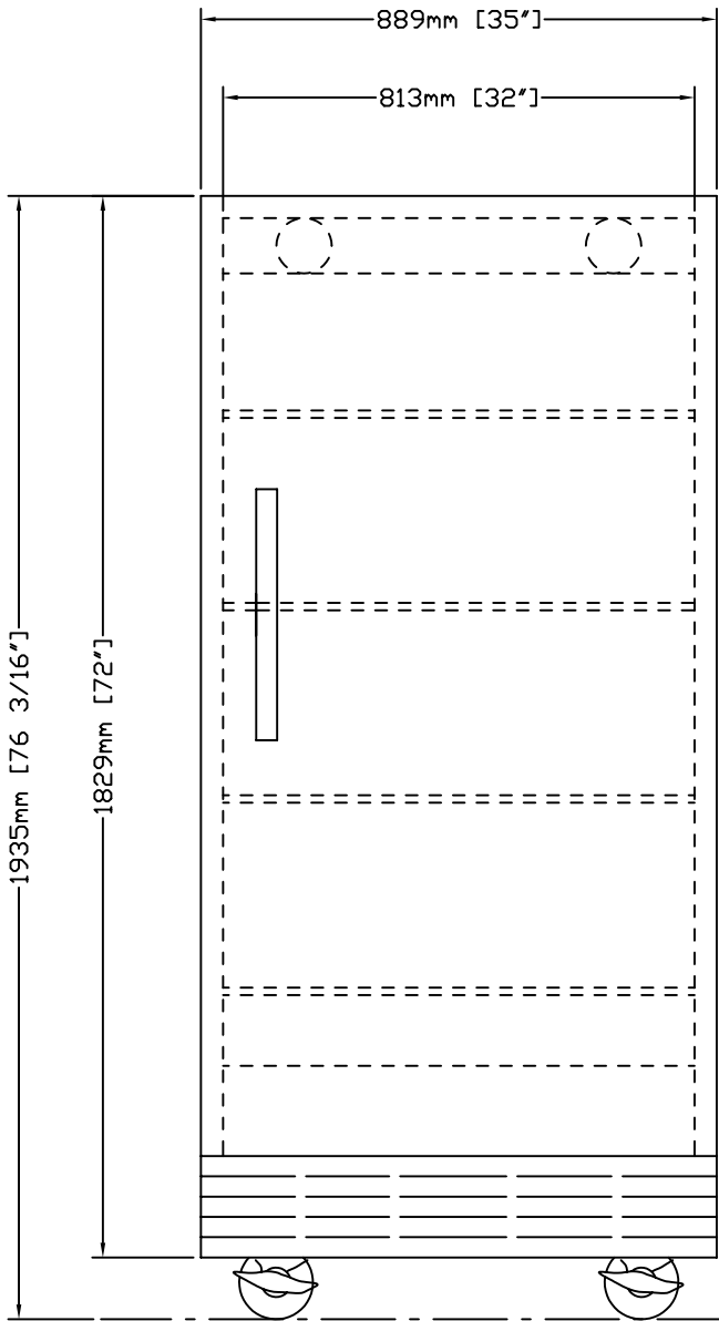
FRONT VIEW
