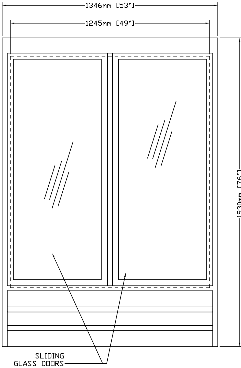
FRONT VIEW
